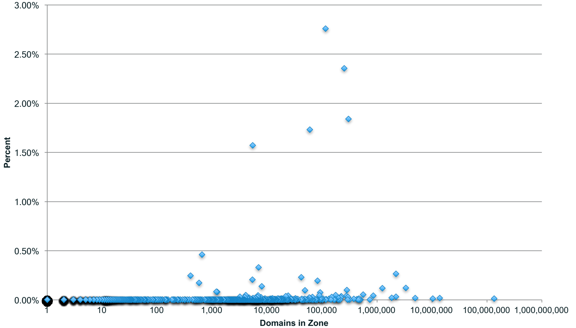
Malware Percentage
